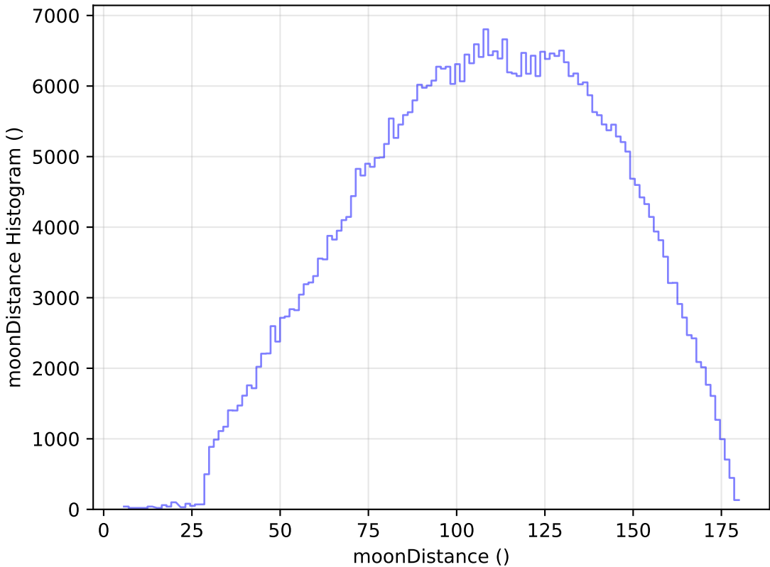
too_ignore_100_1v3.4_10yrs All sky r band: moonDistance Histogram
