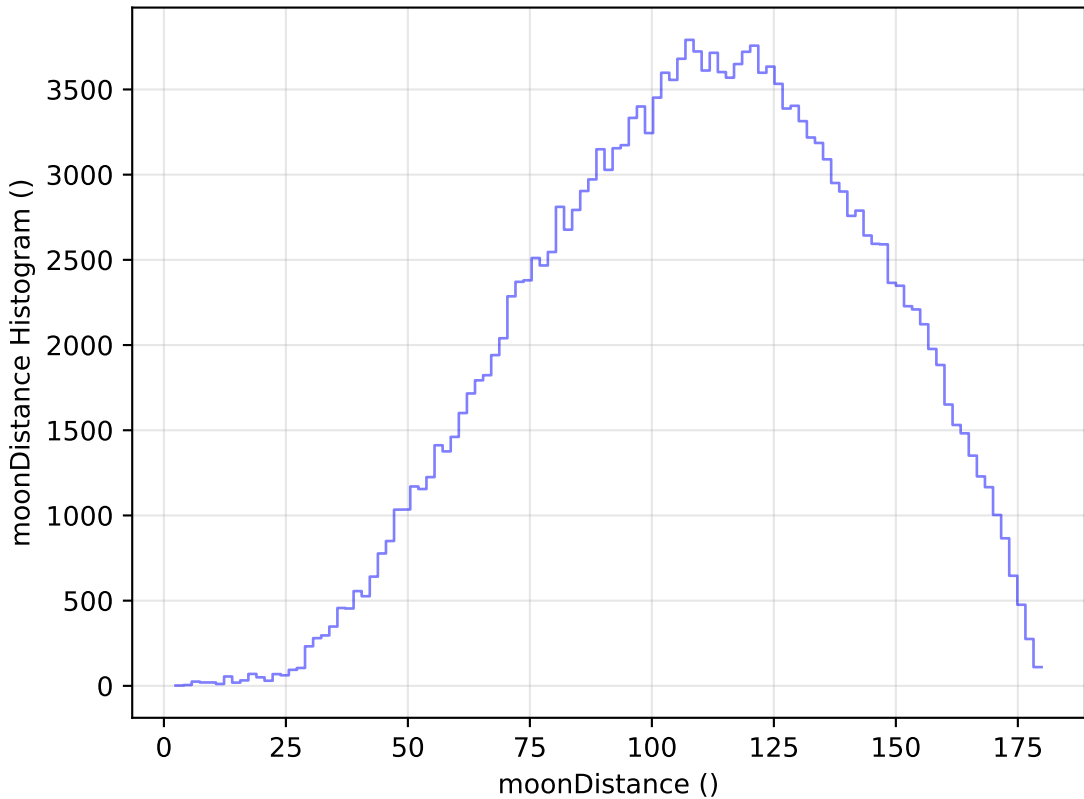
too_ignore_100_1v3.4_10yrs All sky g band: moonDistance Histogram
