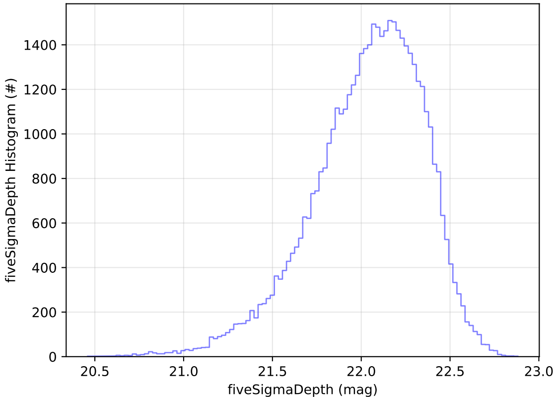
too_ignore_100_1v3.4_10yrs Yr 1 y band: fiveSigmaDepth Histogram
