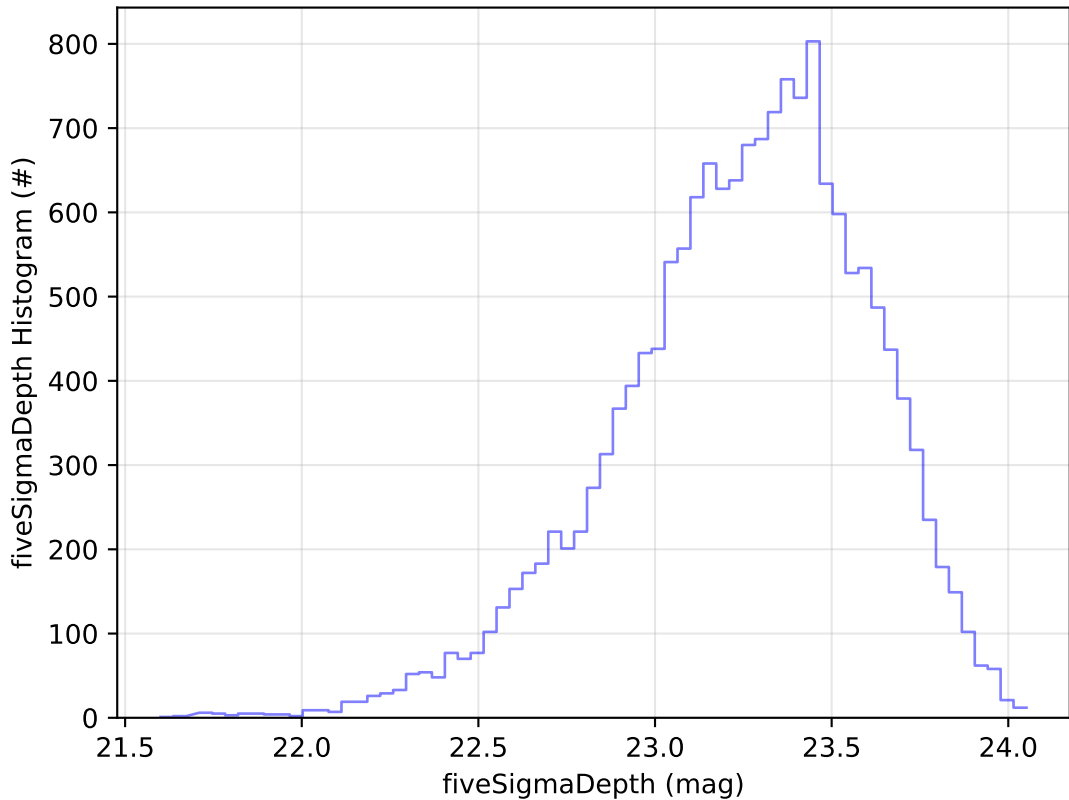
too_ignore_100_1v3.4_10yrs Yr 1 u band: fiveSigmaDepth Histogram
