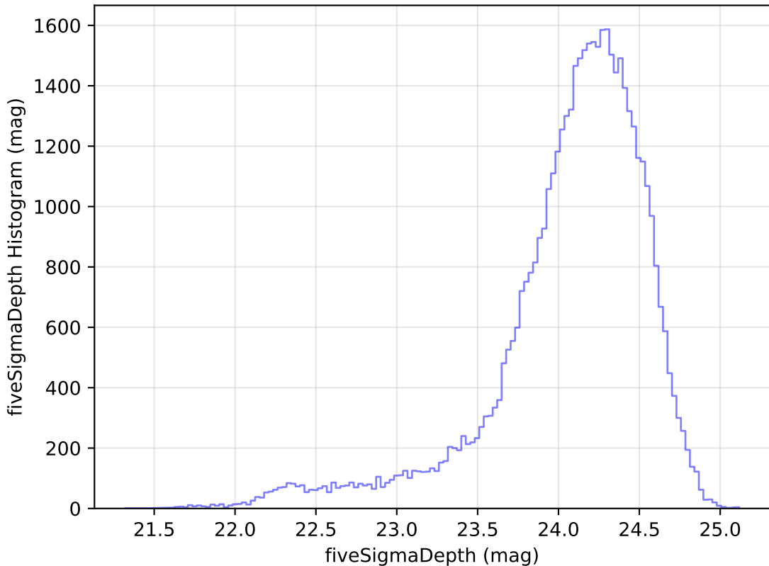
too_ignore_100_1v3.4_10yrs Yr 1 r band: fiveSigmaDepth Histogram
