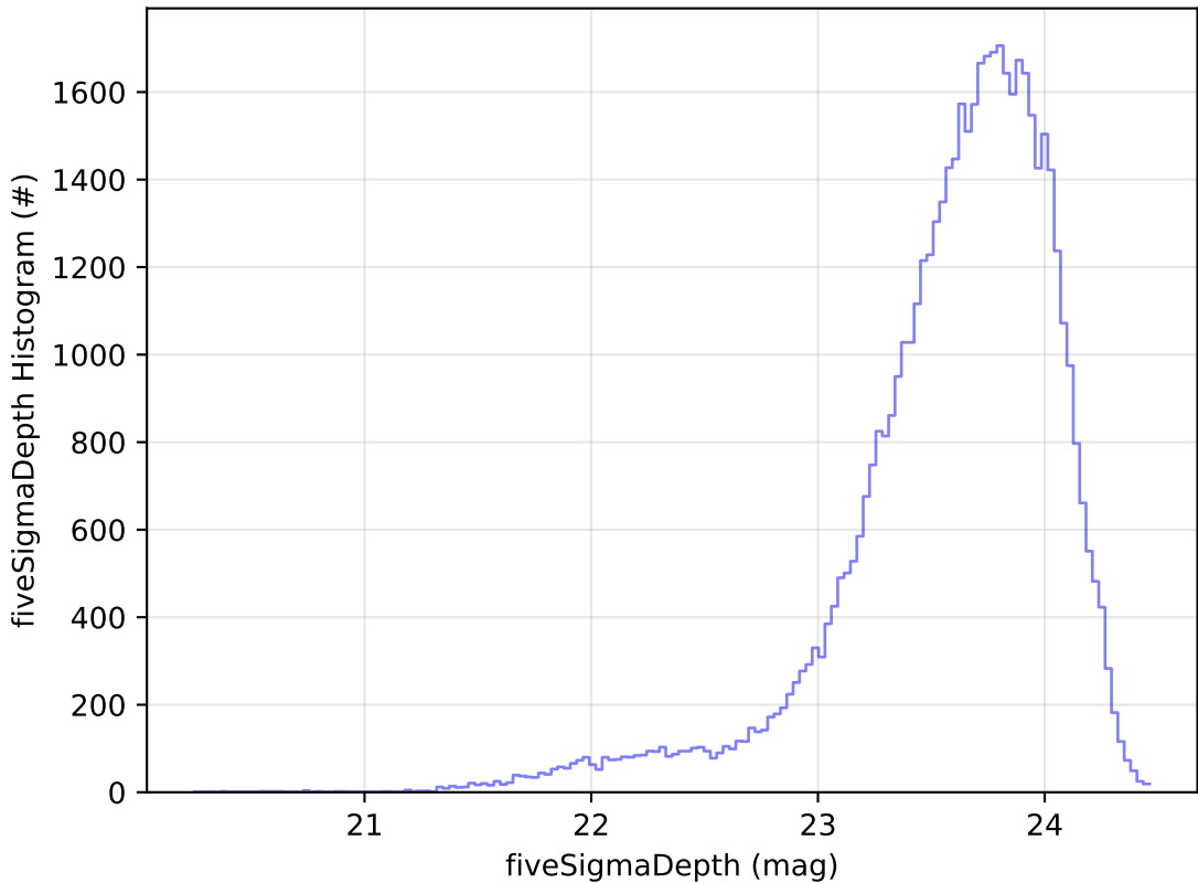
too_ignore_100_1v3.4_10yrs Yr 1 i band: fiveSigmaDepth Histogram
