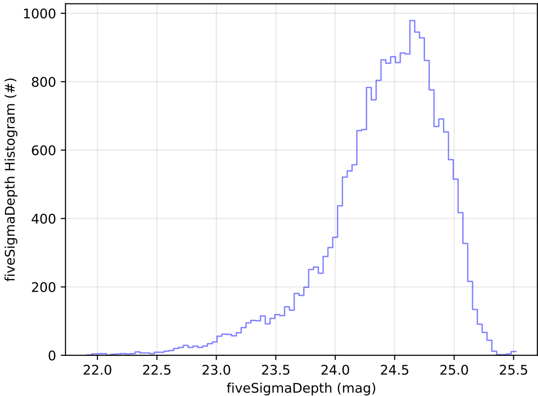
too_ignore_100_1v3.4_10yrs Yr 1 g band: fiveSigmaDepth Histogram
