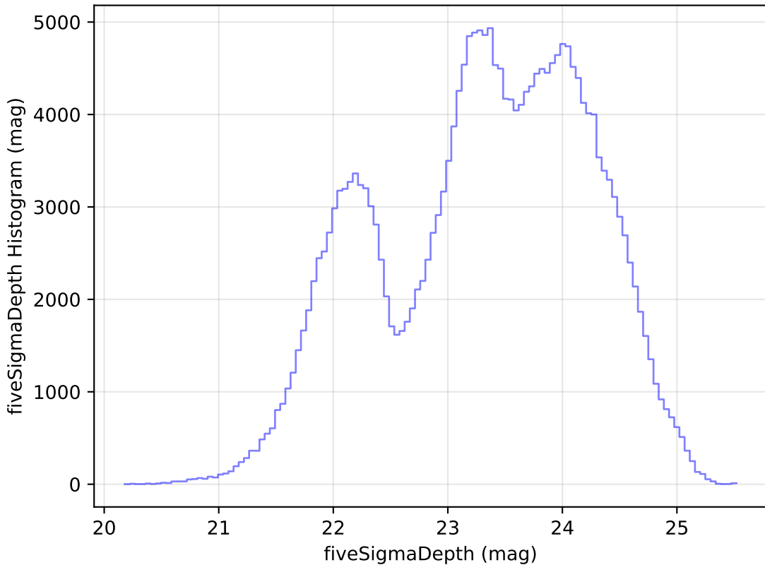
too_ignore_100_1v3.4_10yrs Yr 1 all bands: fiveSigmaDepth Histogram
