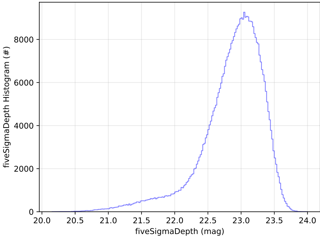
too_ignore_100_1v3.4_10yrs WFD z band: fiveSigmaDepth Histogram
