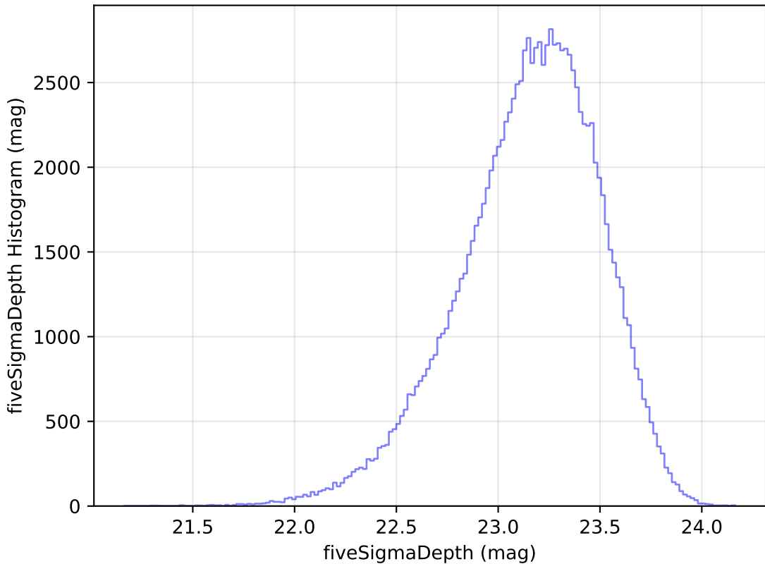
too_ignore_100_1v3.4_10yrs WFD u band: fiveSigmaDepth Histogram
