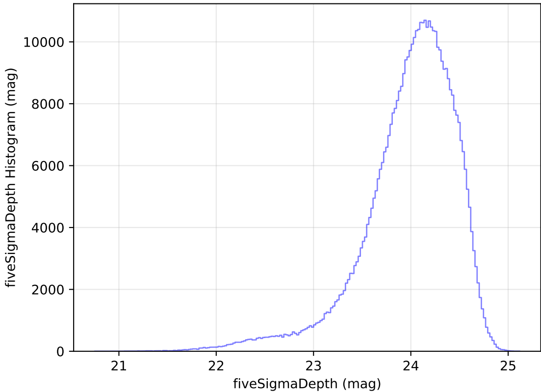
too_ignore_100_1v3.4_10yrs WFD r band: fiveSigmaDepth Histogram
