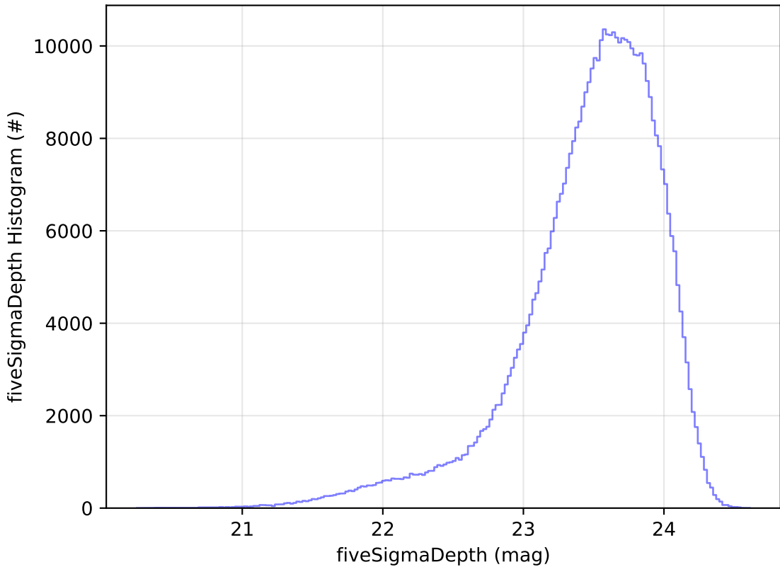
too_ignore_100_1v3.4_10yrs WFD i band: fiveSigmaDepth Histogram
