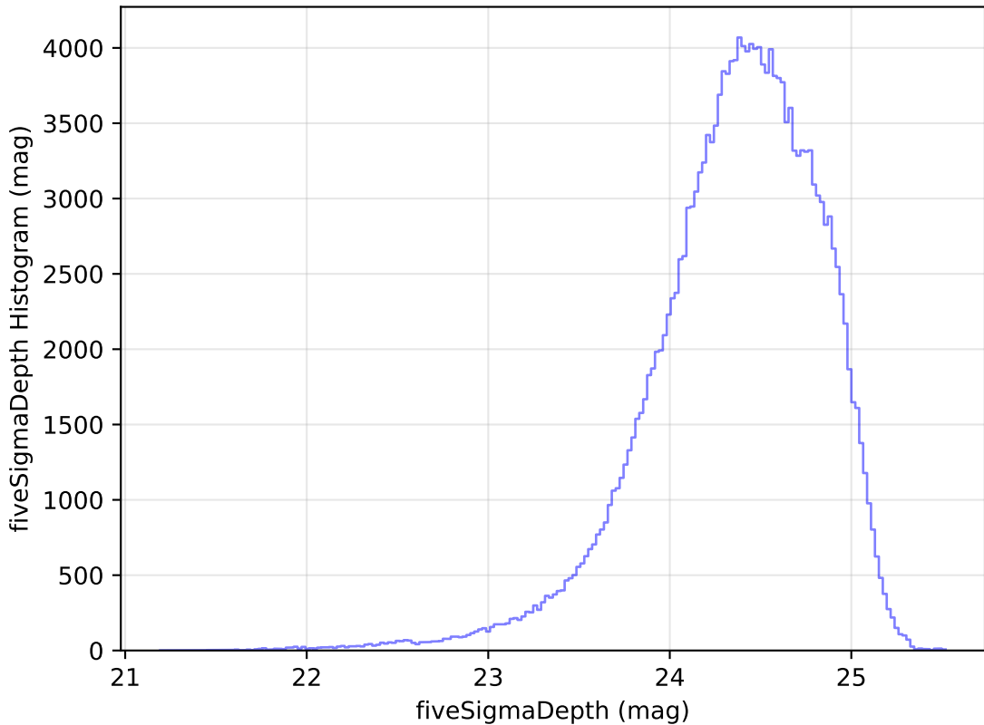
too_ignore_100_1v3.4_10yrs WFD g band: fiveSigmaDepth Histogram
