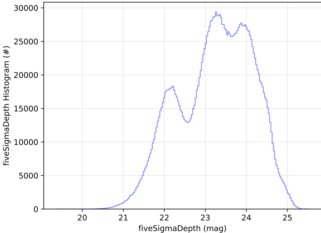
too_ignore_100_1v3.4_10yrs WFD all bands: fiveSigmaDepth Histogram
