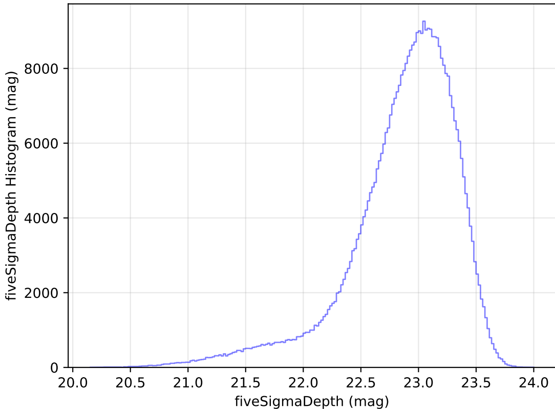
too_ignore_100_1v3.4_10yrs All sky z band: fiveSigmaDepth Histogram
