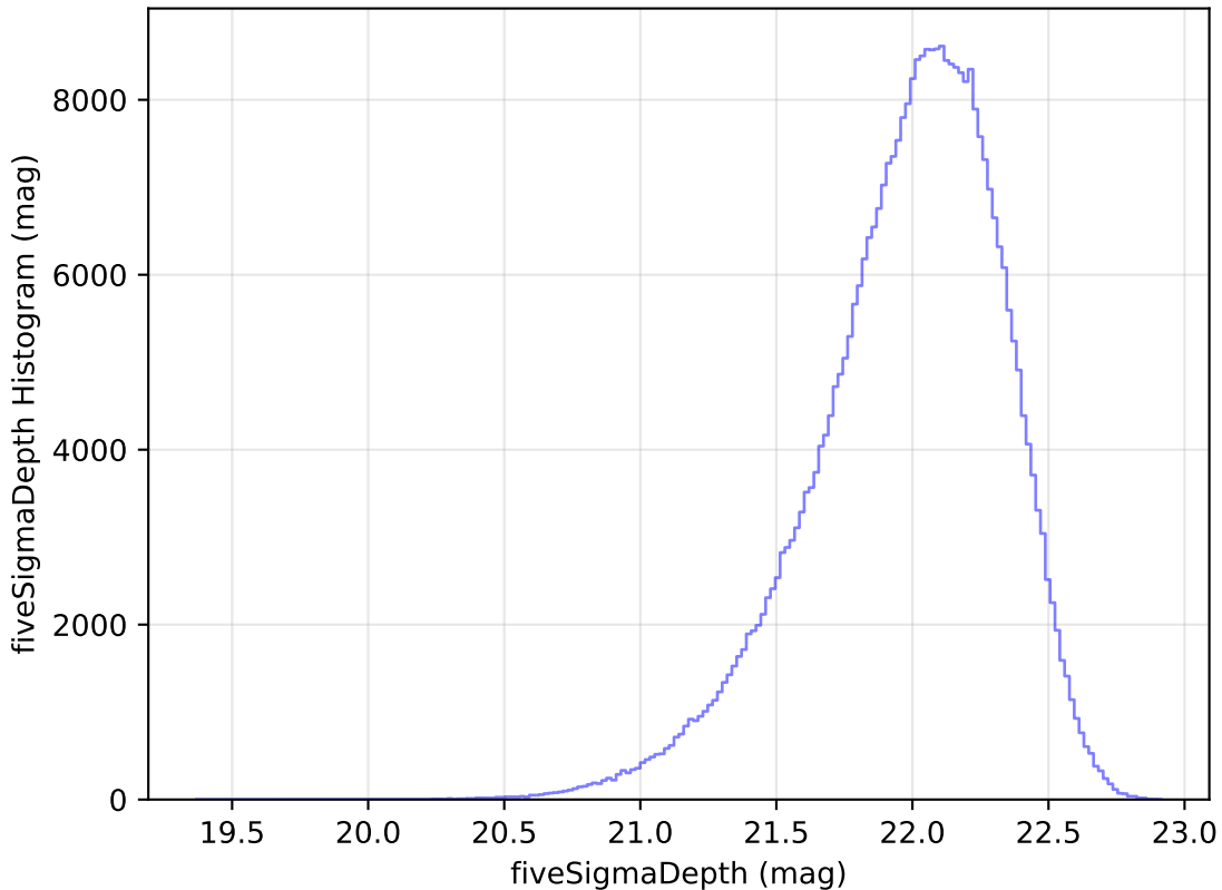
too_ignore_100_1v3.4_10yrs All sky y band: fiveSigmaDepth Histogram
