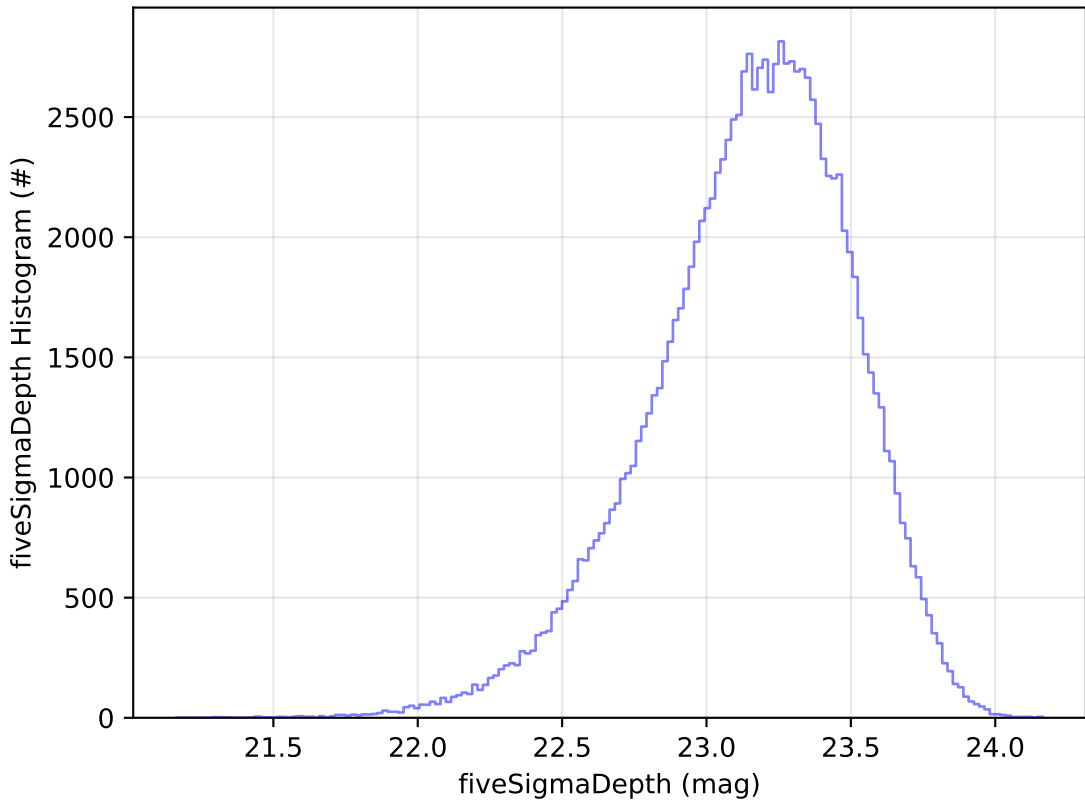
too_ignore_100_1v3.4_10yrs All sky u band: fiveSigmaDepth Histogram
