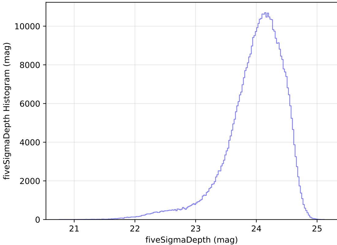
too_ignore_100_1v3.4_10yrs All sky r band: fiveSigmaDepth Histogram
