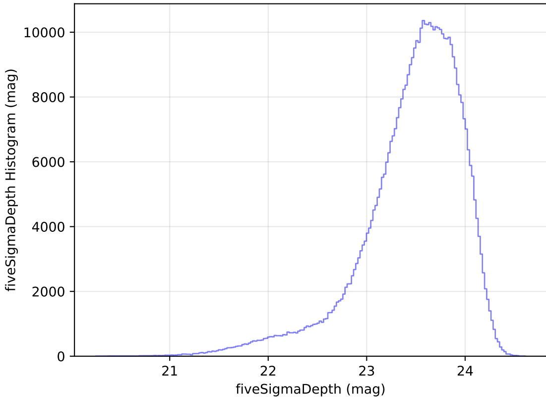
too_ignore_100_1v3.4_10yrs All sky i band: fiveSigmaDepth Histogram
