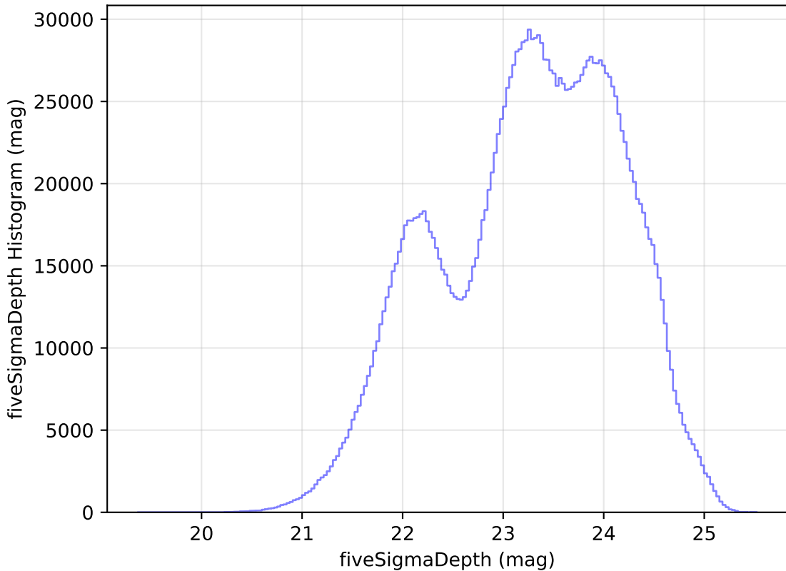
too_ignore_100_1v3.4_10yrs All sky all bands: fiveSigmaDepth Histogram
