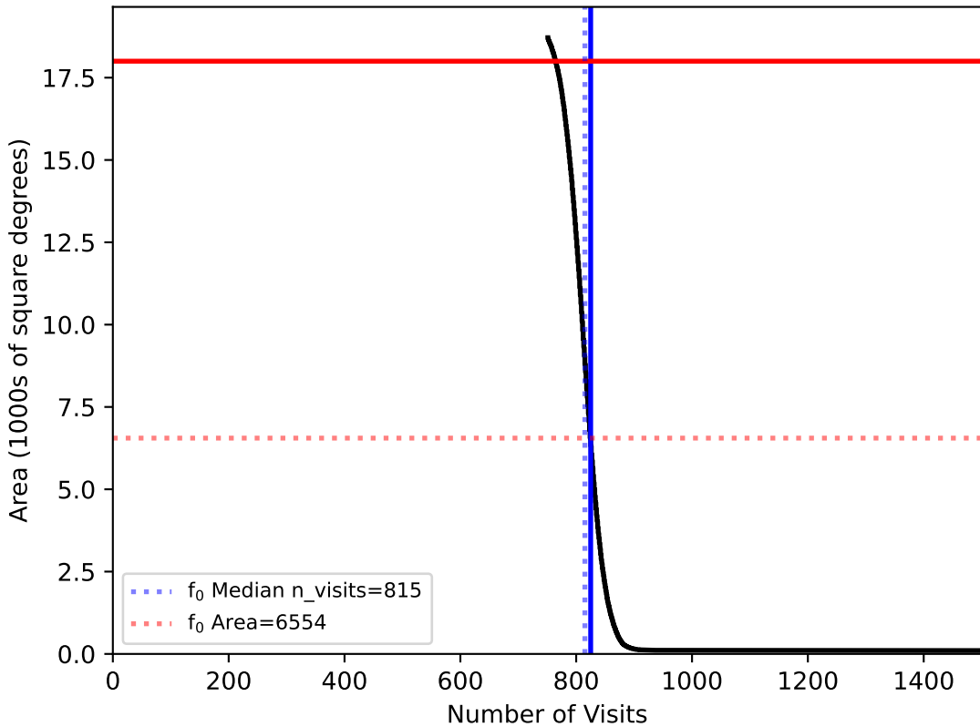
too_ignore_100_1v3.4_10yrs WFD: f0
