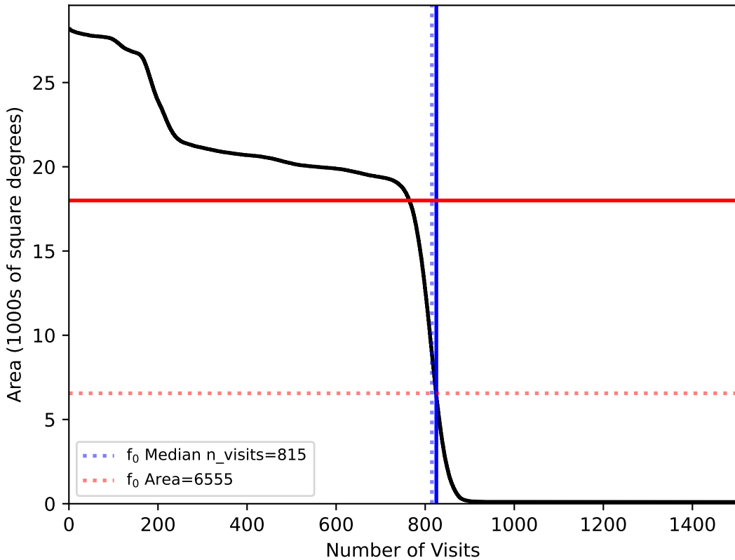
too_ignore_100_1v3.4_10yrs All sky: f 0
