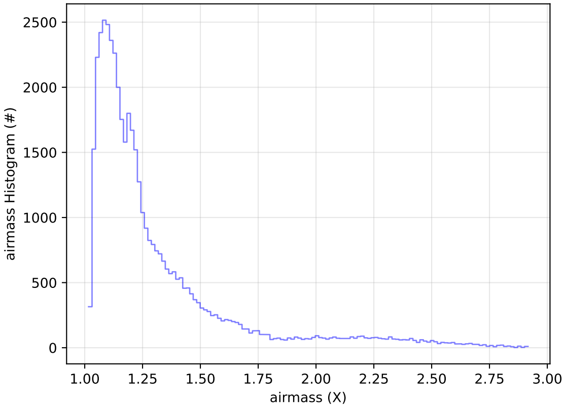
too_ignore_100_1v3.4_10yrs Yr 1 z band: airmass Histogram
