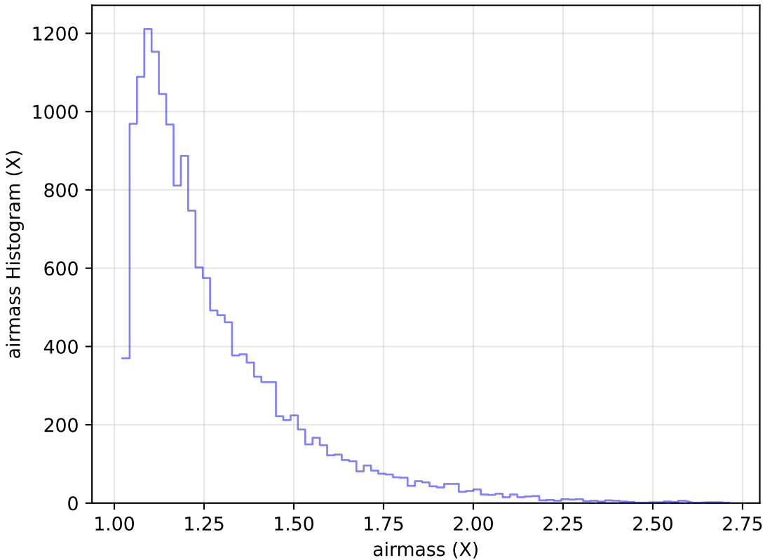
too_ignore_100_1v3.4_10yrs Yr 1 u band: airmass Histogram
