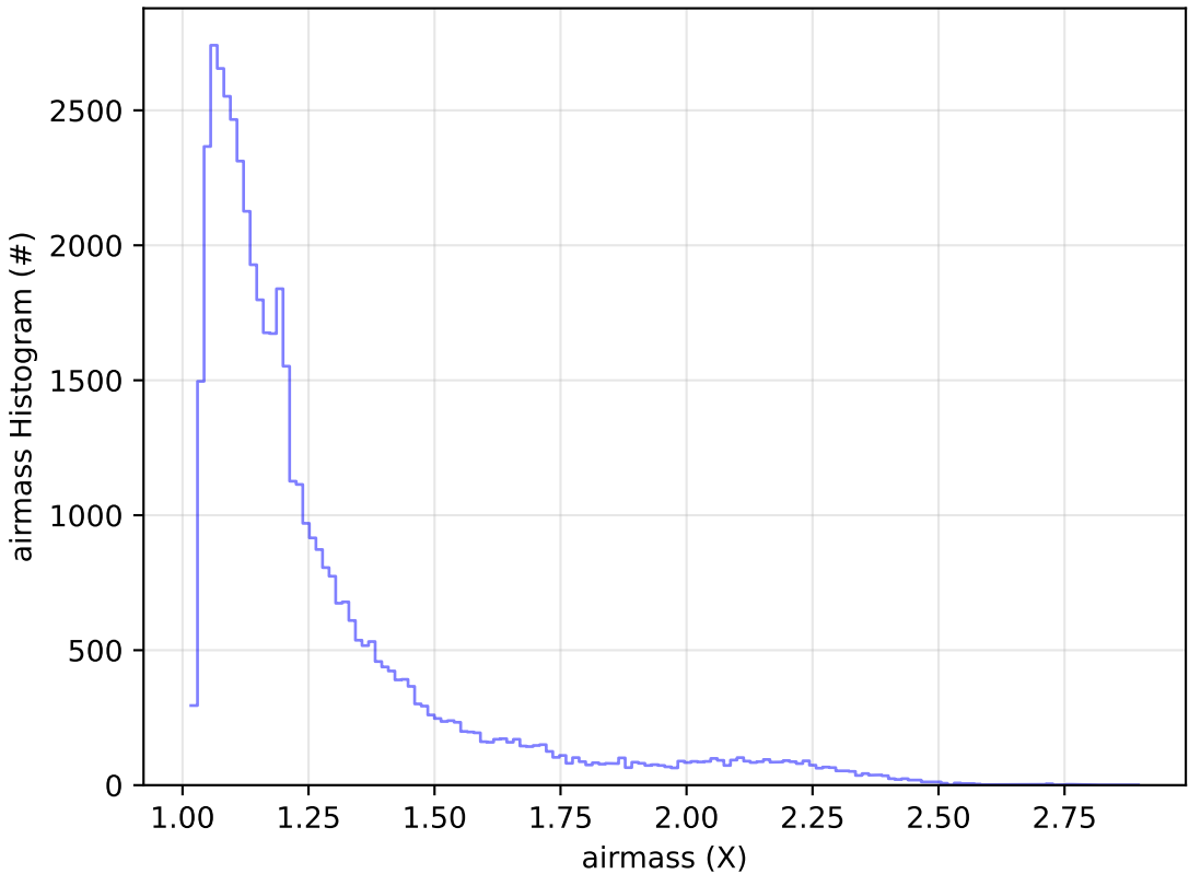
too_ignore_100_1v3.4_10yrs Yr 1 r band: airmass Histogram
