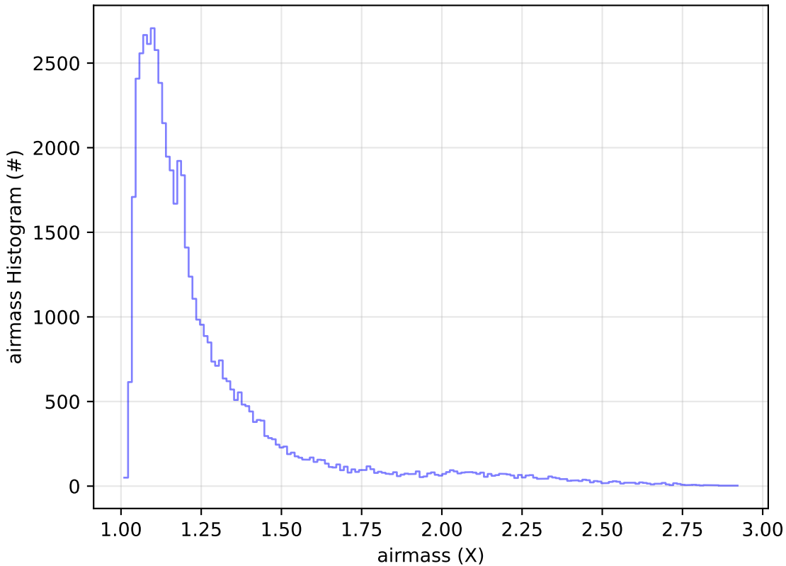
too_ignore_100_1v3.4_10yrs Yr 1 i band: airmass Histogram
