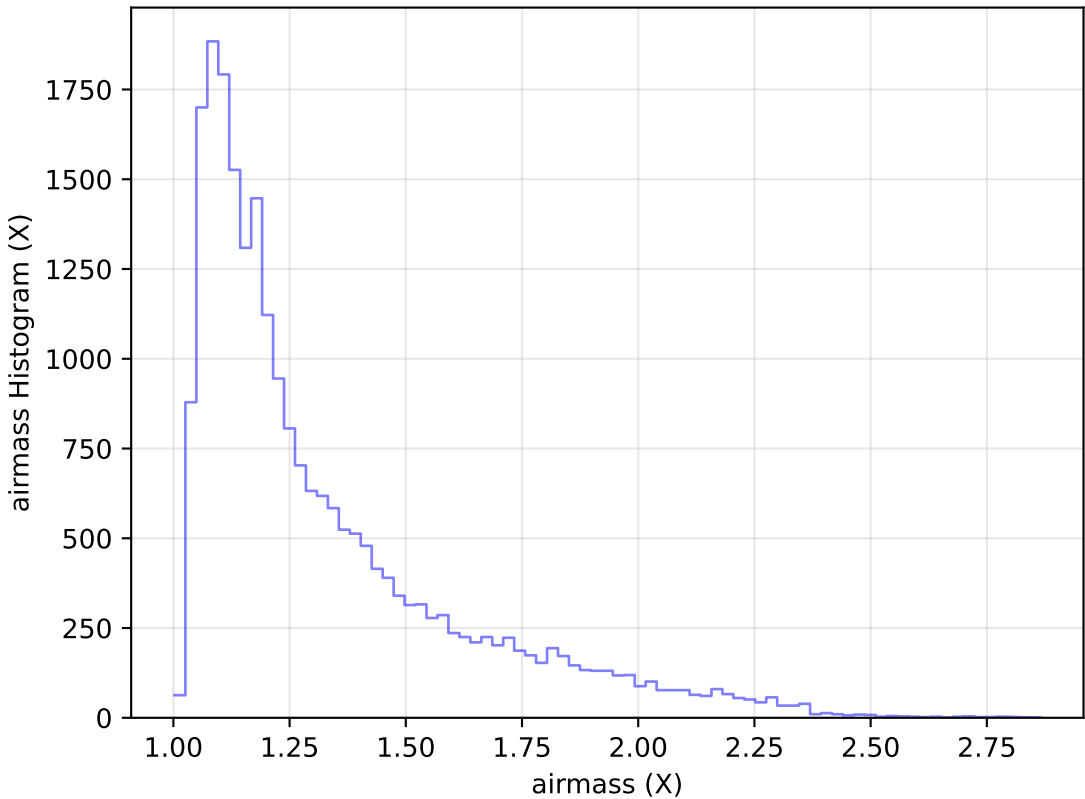
too_ignore_100_1v3.4_10yrs Yr 1 g band: airmass Histogram
