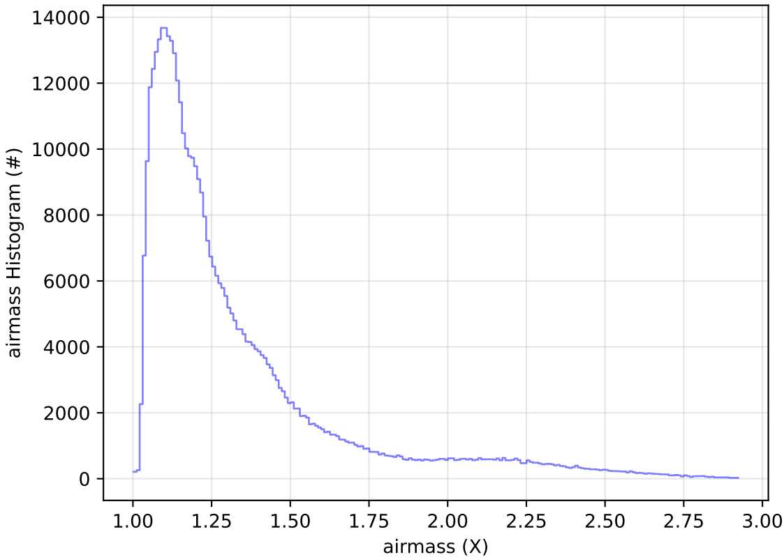
too_ignore_100_1v3.4_10yrs WFD z band: airmass Histogram
