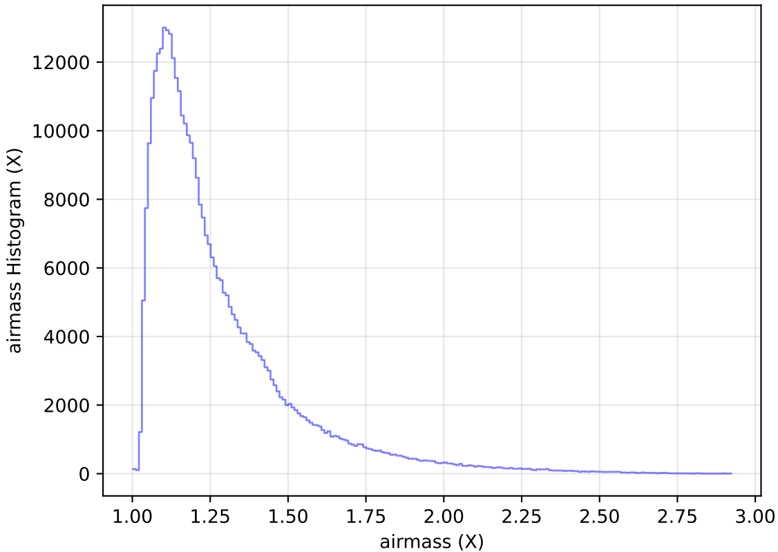
too_ignore_100_1v3.4_10yrs WFD y band: airmass Histogram
