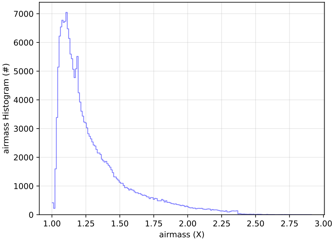
too_ignore_100_1v3.4_10yrs WFD g band: airmass Histogram
