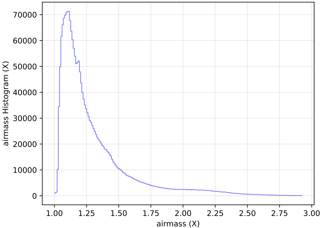
too_ignore_100_1v3.4_10yrs WFD all bands: airmass Histogram
