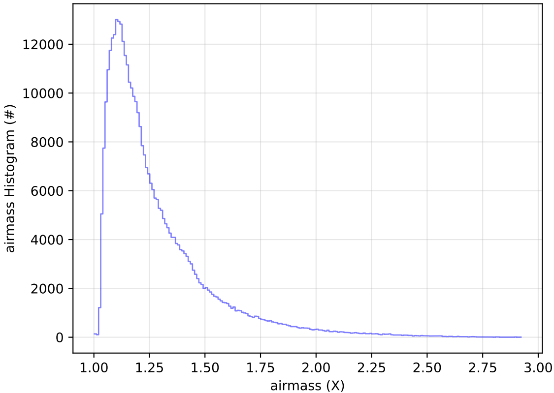
too_ignore_100_1v3.4_10yrs All sky y band: airmass Histogram
