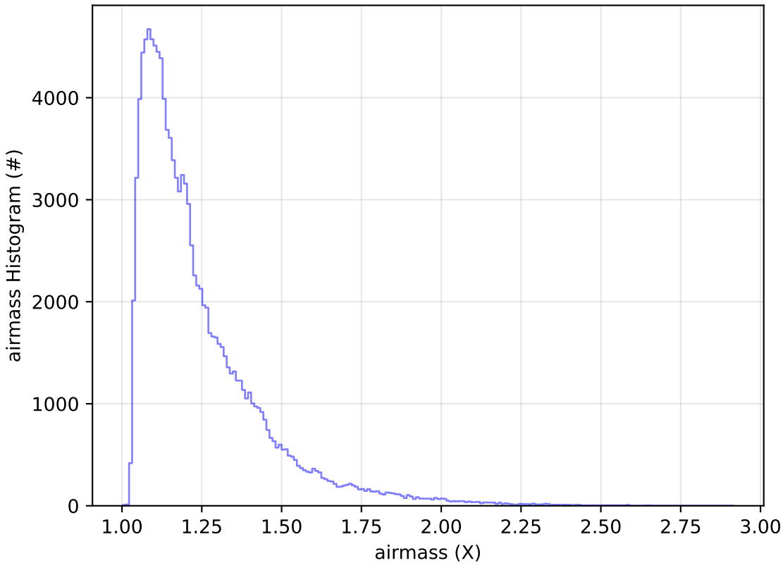
too_ignore_100_1v3.4_10yrs All sky u band: airmass Histogram
