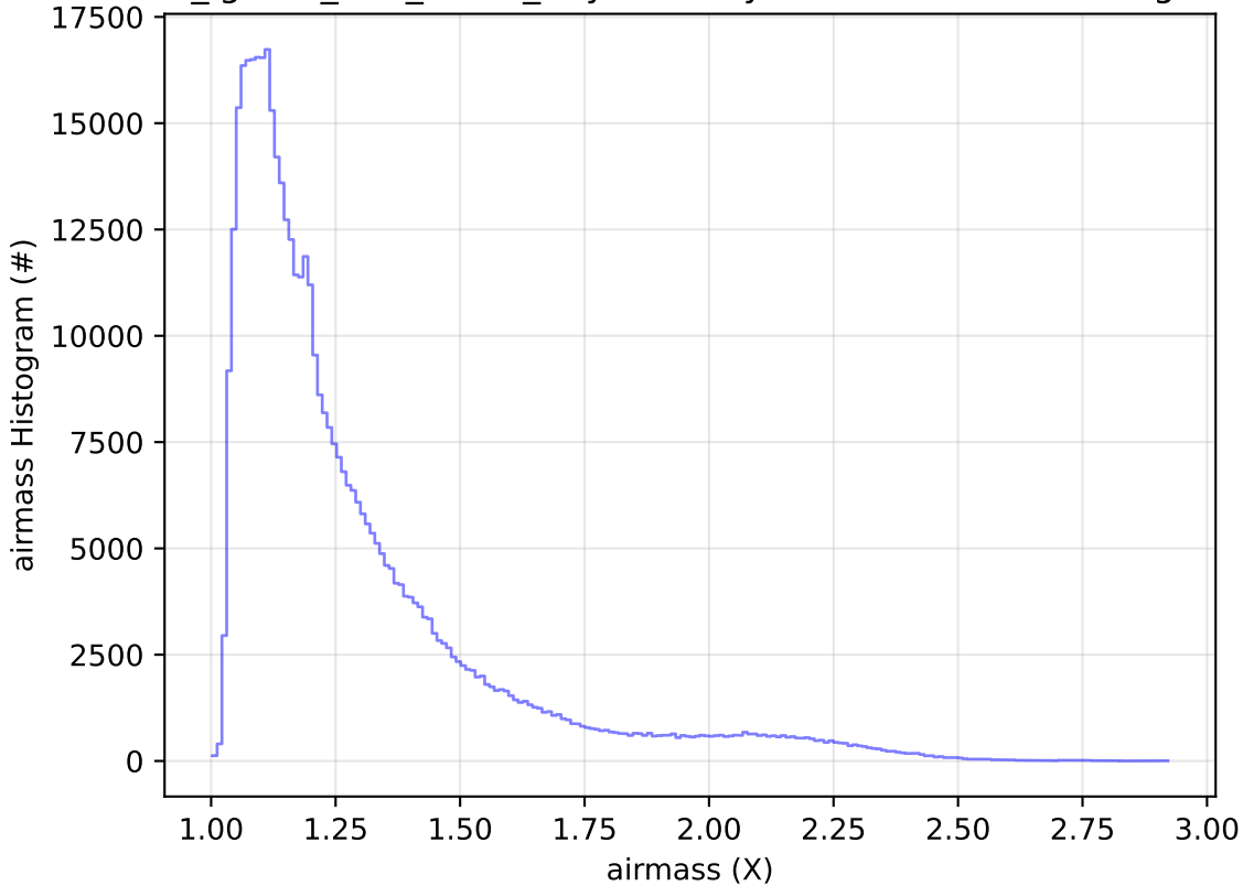
too_ignore_100_1v3.4_10yrs All sky r band: airmass Histogram
