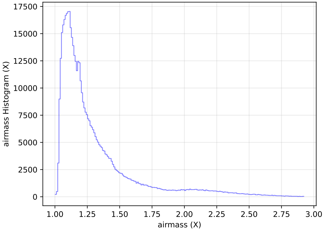
too_ignore_100_1v3.4_10yrs All sky i band: airmass Histogram
