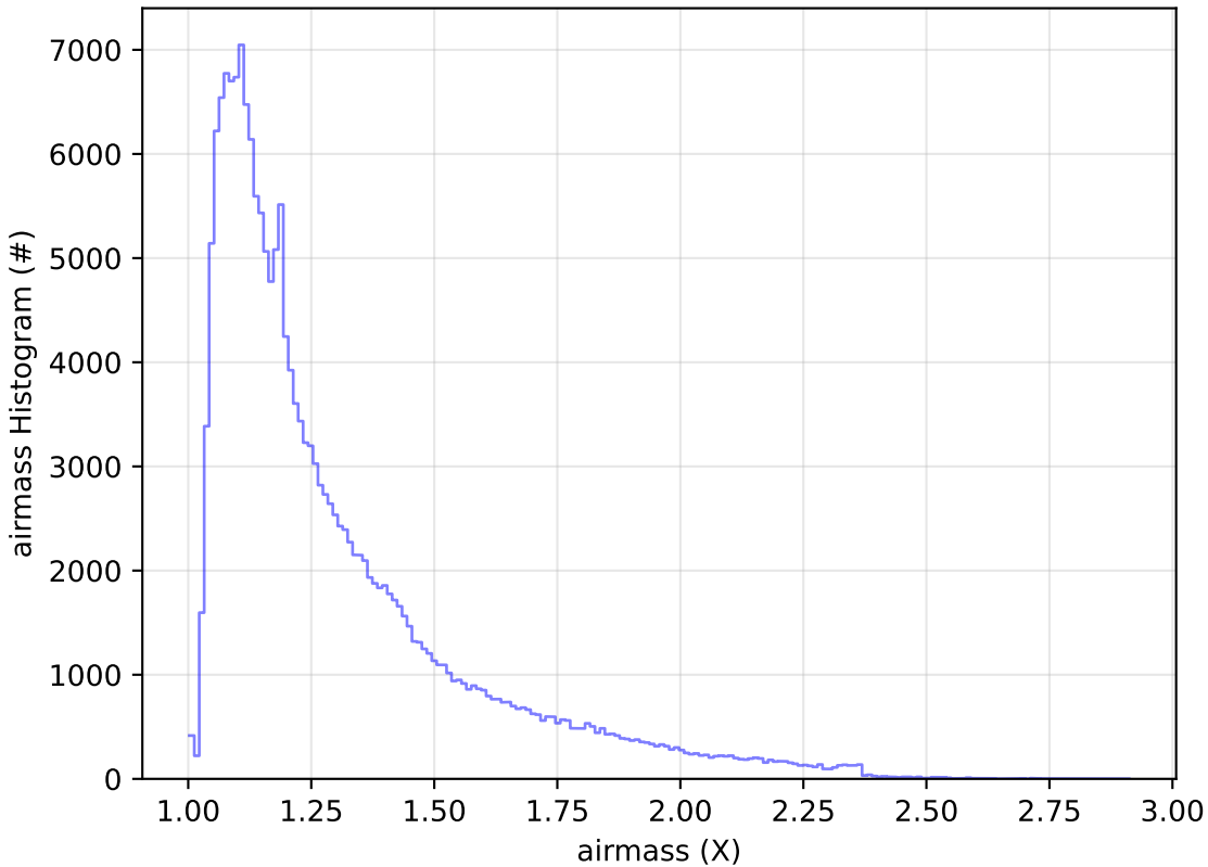
too_ignore_100_1v3.4_10yrs All sky g band: airmass Histogram
