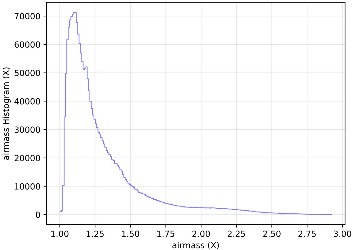
too_ignore_100_1v3.4_10yrs All sky all bands: airmass Histogram
