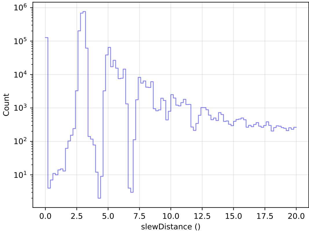
too_ignore_100_1v3.4_10yrs All visits: Zoom Slew Distance Histogram
