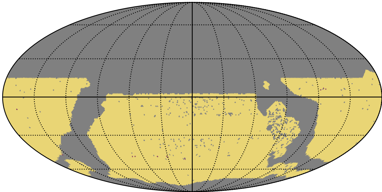
too_ignore_100_1v3.4_10yrs WFD: RapidRevisits
