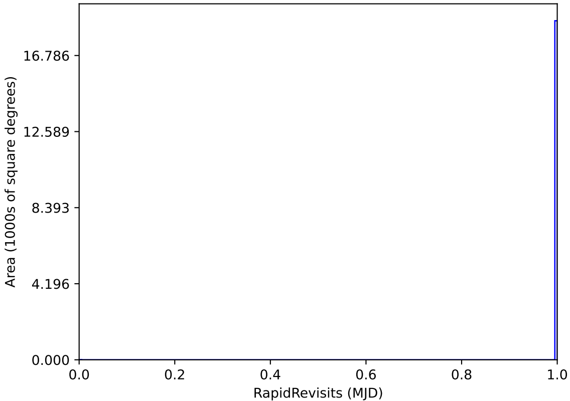
too_ignore_100_1v3.4_10yrs WFD: RapidRevisits
