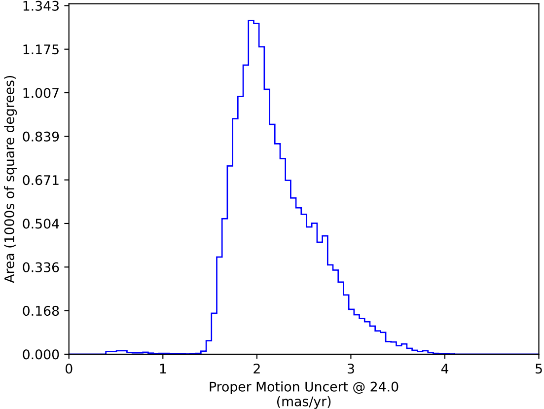
too_ignore_100_1v3.4_10yrs WFD: Proper Motion Uncert @ 24.0
