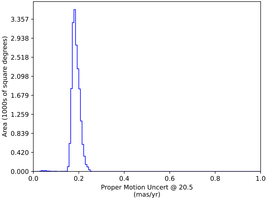
too_ignore_100_1v3.4_10yrs WFD: Proper Motion Uncert @ 20.5
