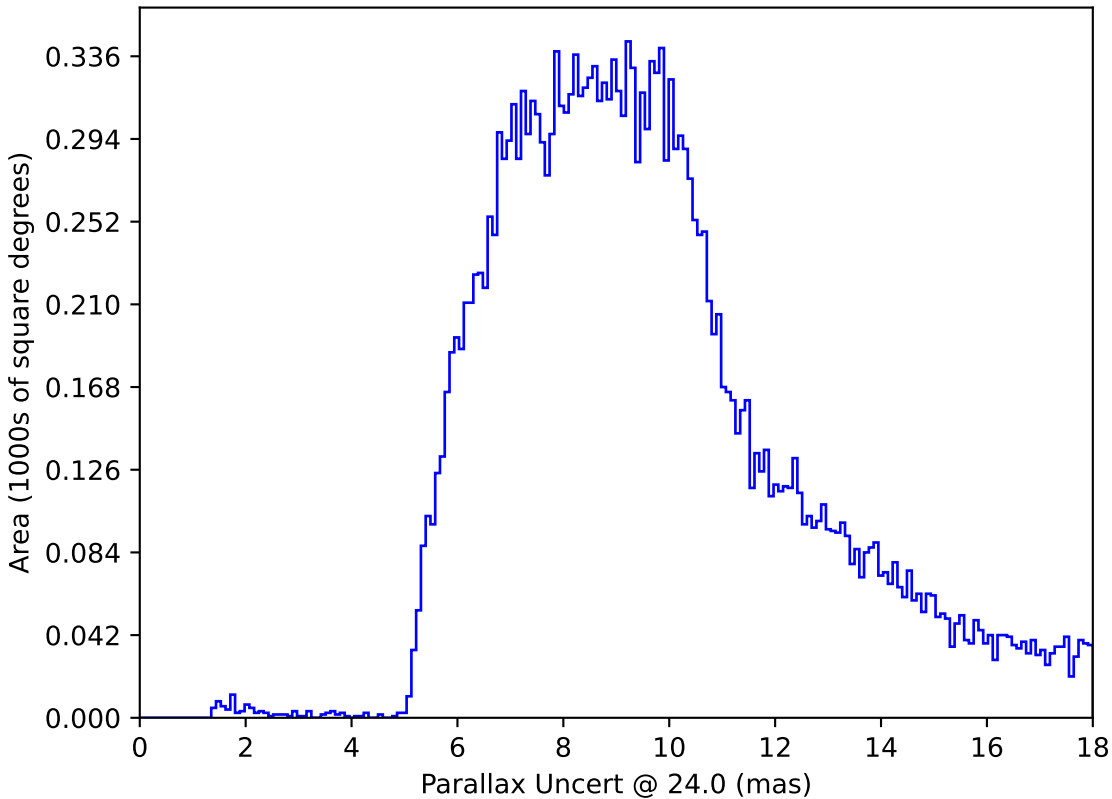
too_ignore_100_1v3.4_10yrs All sky: Parallax Uncert @ 24.0
