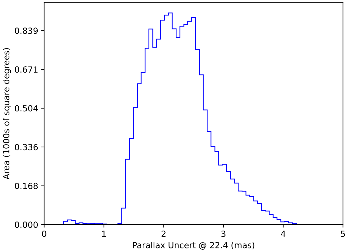
too_ignore_100_1v3.4_10yrs WFD: Parallax Uncert @ 22.4
