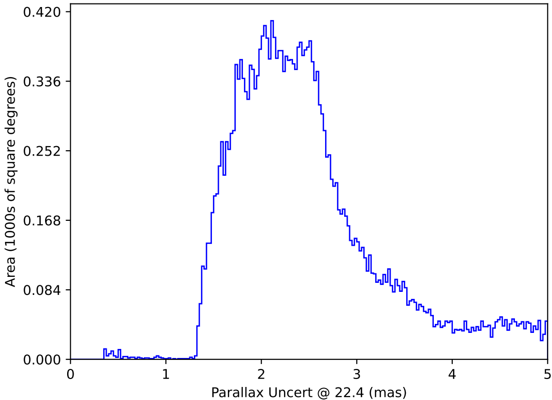
too_ignore_100_1v3.4_10yrs All sky: Parallax Uncert @ 22.4
