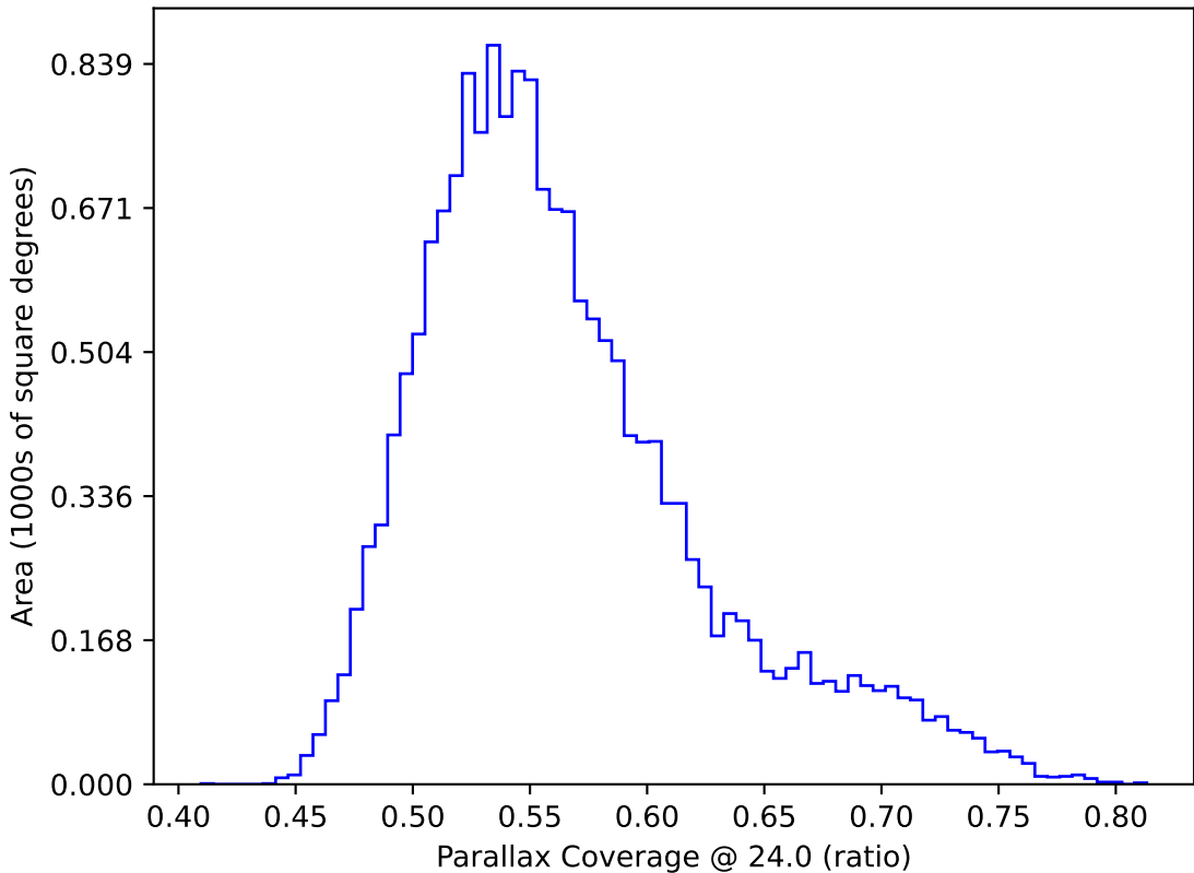
too_ignore_100_1v3.4_10yrs WFD: Parallax Coverage @ 24.0
