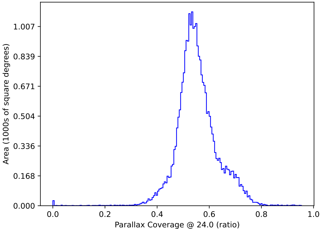
too_ignore_100_1v3.4_10yrs All sky: Parallax Coverage @ 24.0
