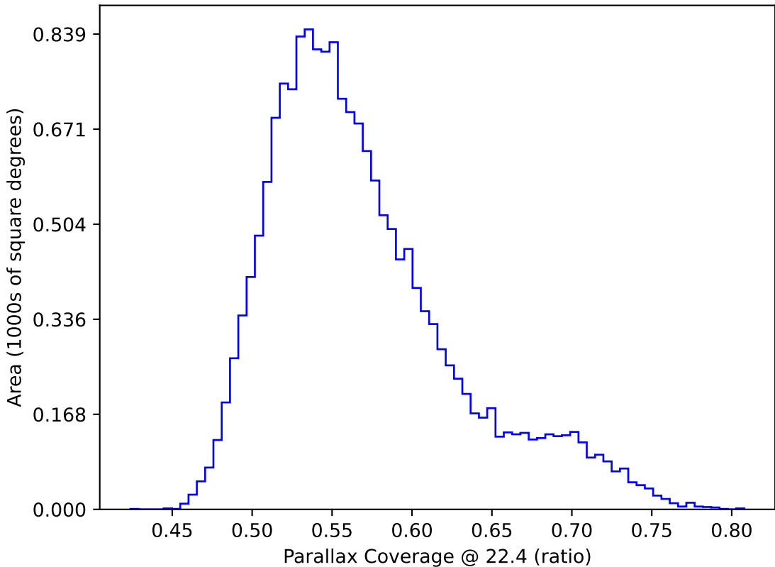
too_ignore_100_1v3.4_10yrs WFD: Parallax Coverage @ 22.4
