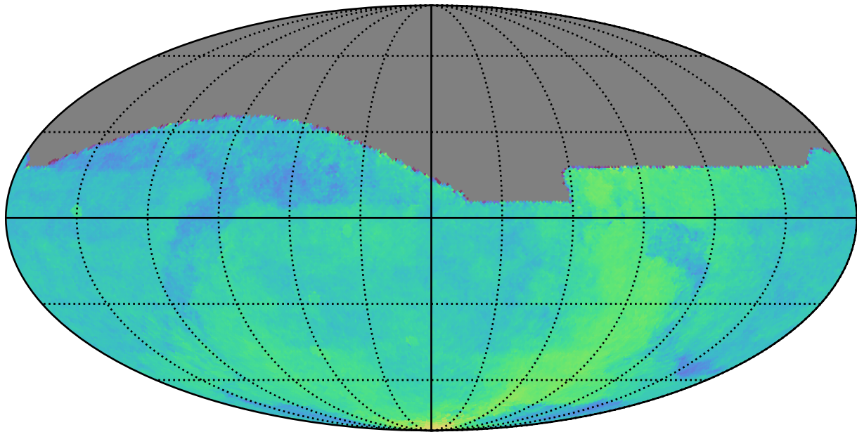
too_ignore_100_1v3.4_10yrs All sky: Parallax Coverage @ 22.4
