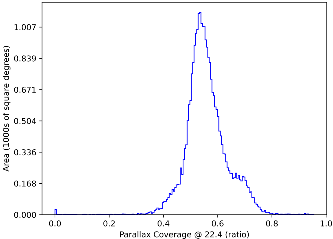
too_ignore_100_1v3.4_10yrs All sky: Parallax Coverage @ 22.4
